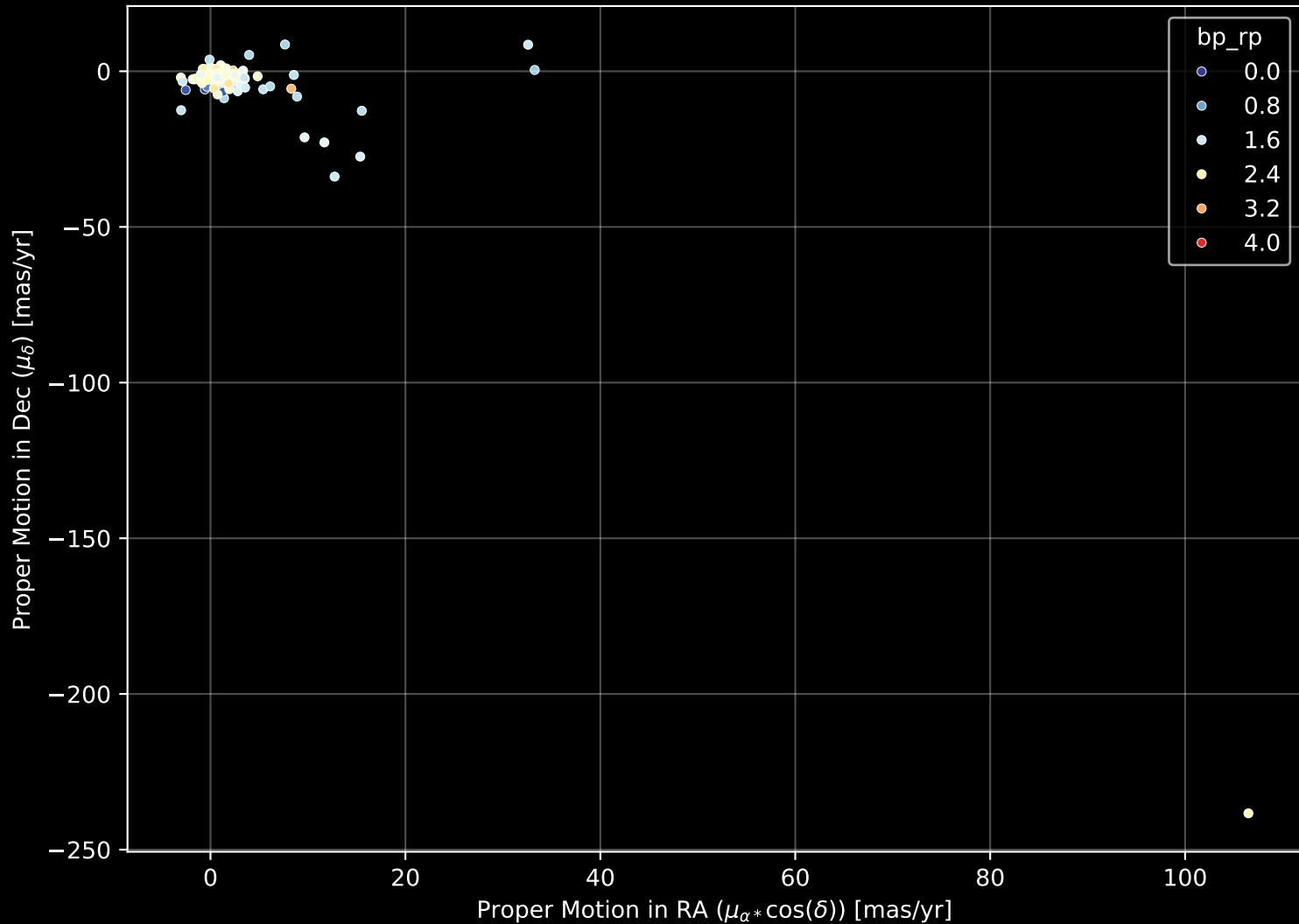
APOGEE DR17 Field: [184-04] Proper Motion Diagram (n= 157)
