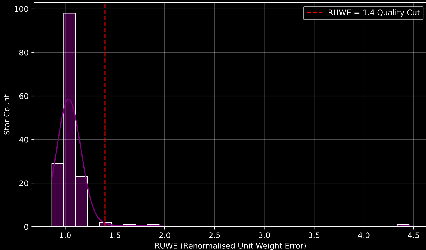
GAPOGEE DR17 Field [184-04] RUWE Distribution (n= 155)
