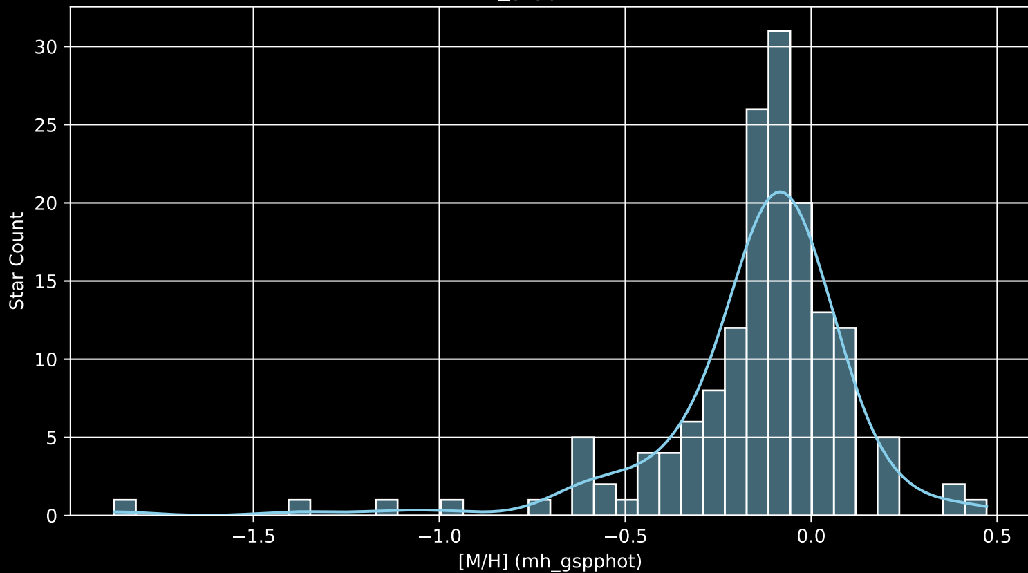
APOGEE DR17 Field: [184-04 [M/H] (mh_gspphot) (n= 157)
