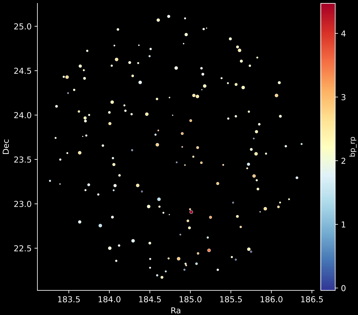
APOGEE DR17 Field: [184-04] Stars: 157
