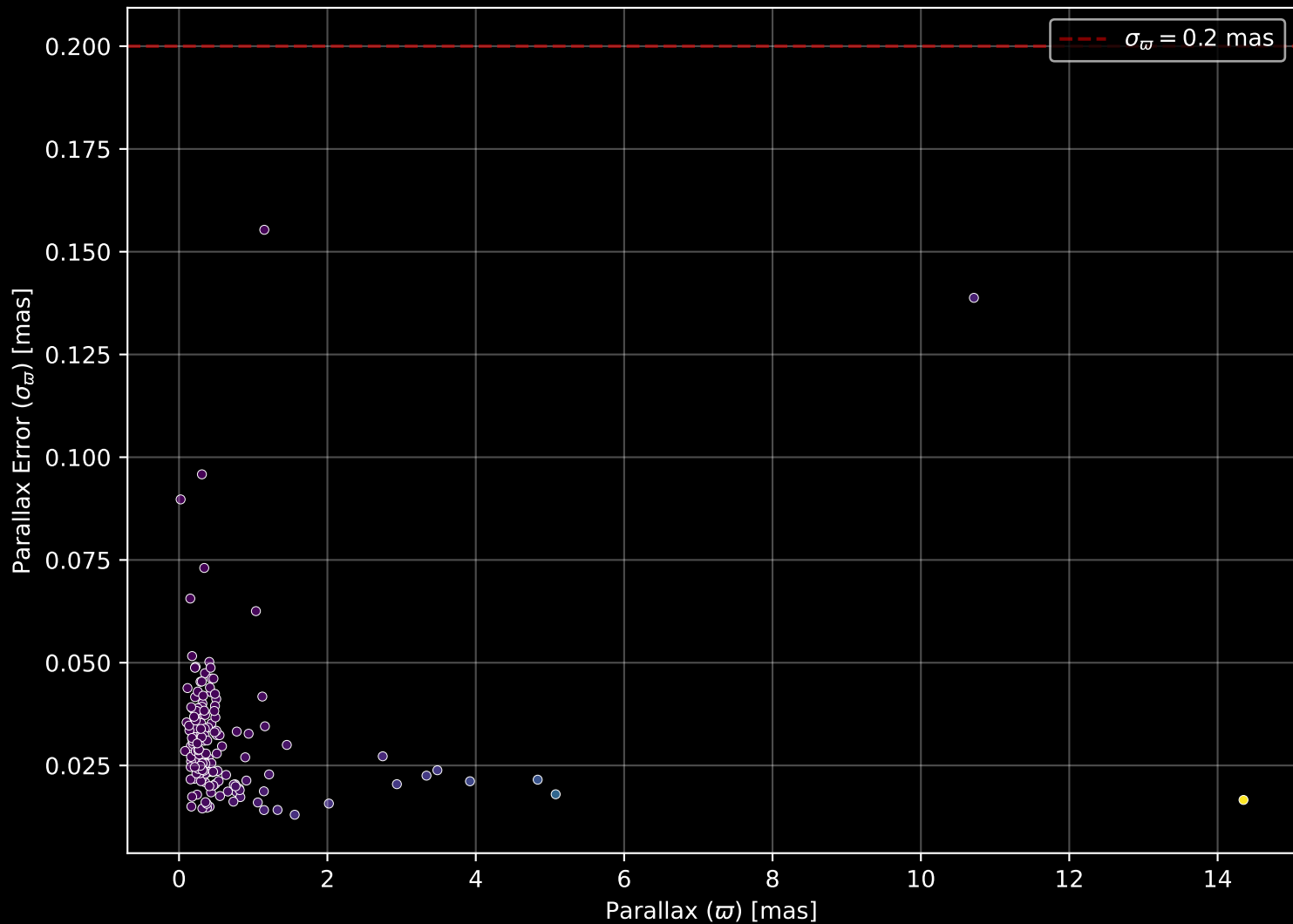
APOGEE DR17 Field: [184-04] Parallax Quality (n= 157)
